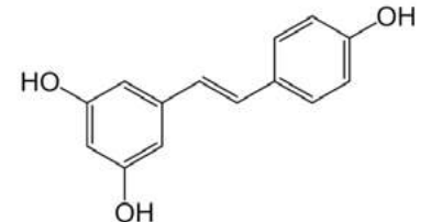
Resveratrol
