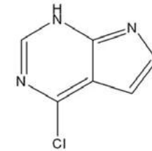
4-Chloropyrrolo[2,3-d]pyrimidine
