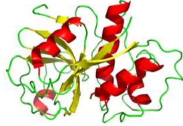
Papain
