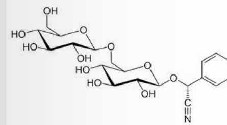
Amygdalin
