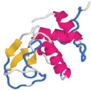
Lysozyme hydrochloride
