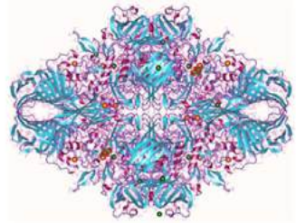
Lactase
