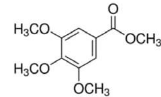
Methyl 3,4,5-trimethoxybenzoate
