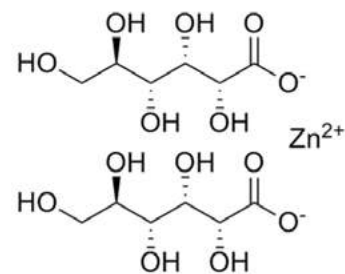
Zinc Gluconate
