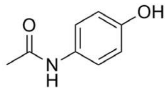
Paracetamol
