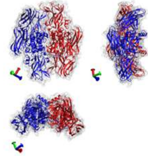
Transglutaminase
