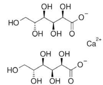
Calcium Gluconate
